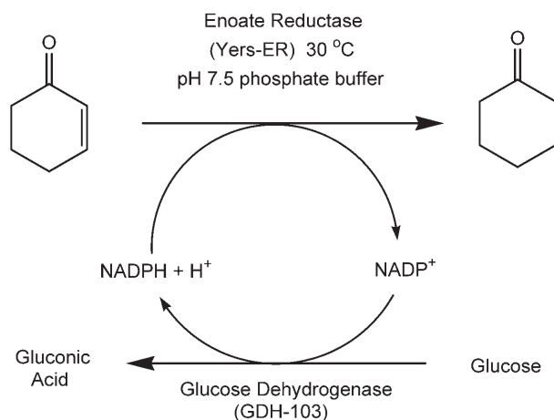
Scheme 1. Enzyme-coupled cofactor regeneration system with enoate reductase from Yersinia bercovieri and glucose dehydrogenase (GDH-103).
