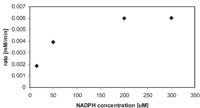
Figure 5. Determining the saturation concentration of NADPH for Yers-ER. Assay conditions: 25 °C, pH 7.5, 10 mM 2-cyclohexen-1-one.
