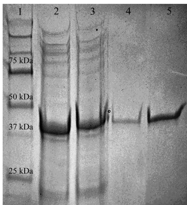
Figure 2. SDS-PAGE of each step in the \text{Ni}^{2+} -NTA purification of the ER from Yersinia bercovieri . The standard protocol was used from QIAGEN with \text{Ni}^{2+} -NTA beads. Lane 1: ladder; lane 2: cell lysate, lane 3: flow through from the binding solution; lane 4: flow through from the wash buffer; lane 5: eluted fraction.
