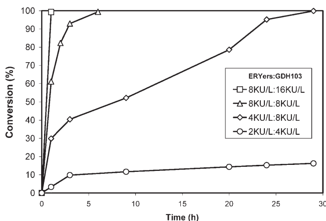
Figure 6. Enzymatic oxidation of 25 g/L of 2-cyclohexen-1-one to 2-cyclohexanone at 30 °C in 200 mM phosphate pH 7.5.
