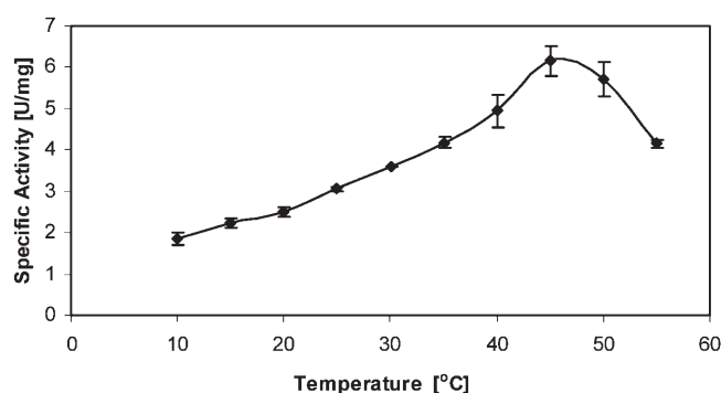
Figure 3. Activity-temperature profile of Yers-ER. The samples were heated immediately before the assay and contained extra NADPH (250 μM) to ensure saturation with reduced enzyme at the start of the run. The buffer contained 200 mM sodium phosphate buffer at pH 7.5, 5 mM 2-cyclohexen-1-one and 200 μM NADPH.
