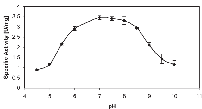
Figure 4. Activity-pH profile of Yers-ER. The measurements were conducted in buffered solution (see Experimental Section) at 25 °C with 5 mM 2-cyclohexen-1-one and 200 μM NADPH.
